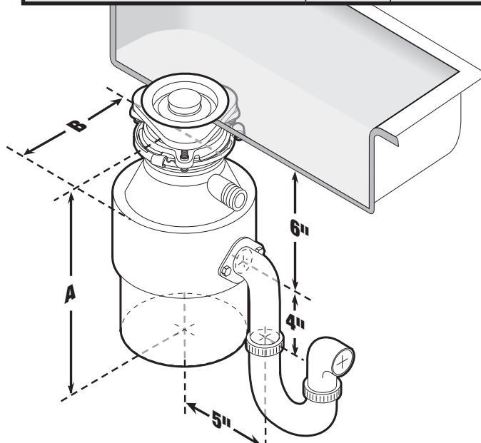
Dimensions/Dimensiones/Dimensions
